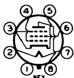
BOTTOM VIEW (8BK)
